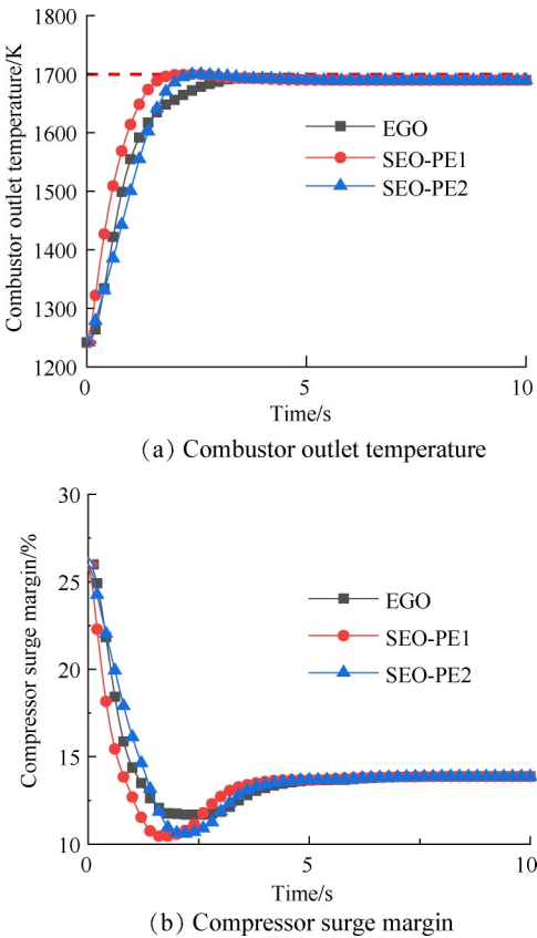
Fig. 3 Optimization results of engine acceleration process
